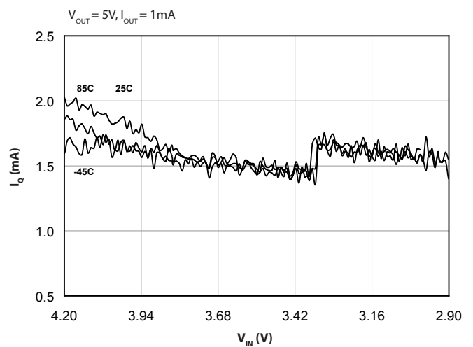
Quiescent Current
